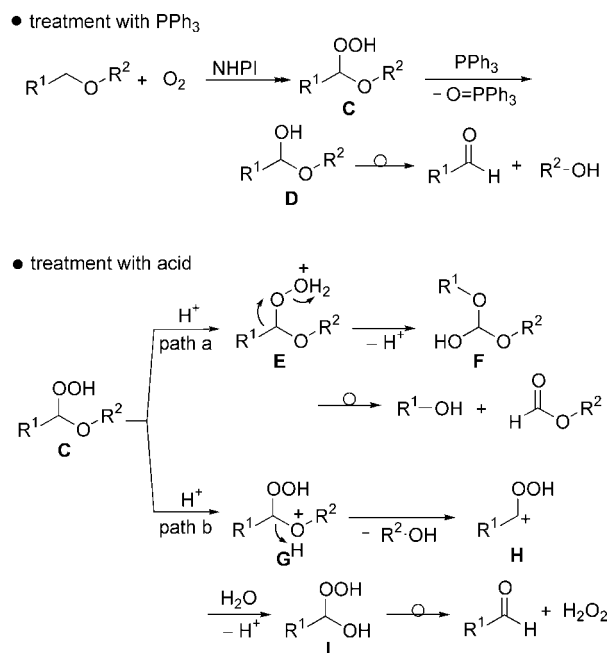
Scheme 2. A possible reaction path for aerobic oxidation of ethers catalyzed by NHPI followed by treatment with \text{PPh}_3 or acid.
